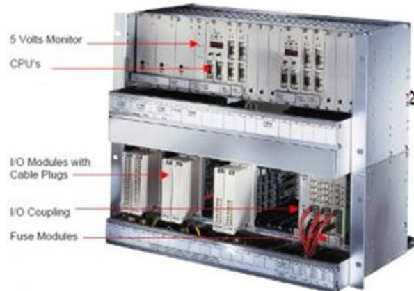
A HIMA HS1q system with I/O rack and I/O modules.
